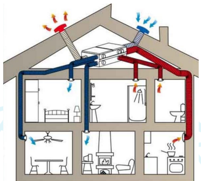
HRV/ERV air flow diagram
