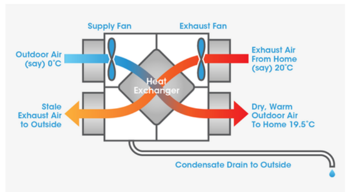
HRV/ERV system diagram
